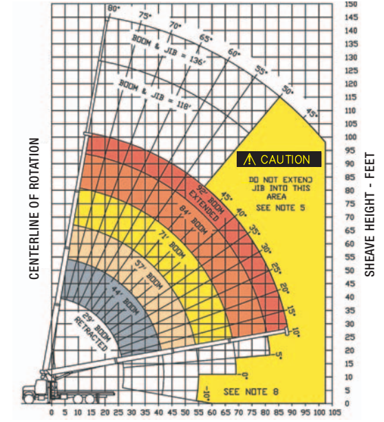
RANGE DIAGRAM (29 - 92 FT BOOM)
