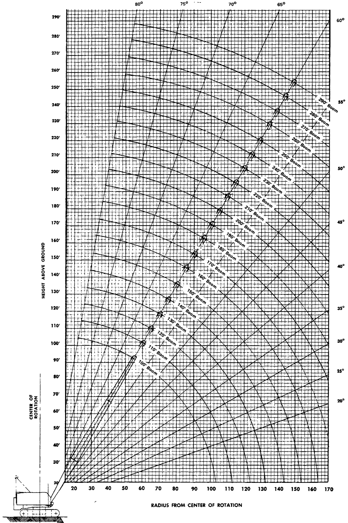
AMERICAN MODEL 9299 CRAWLER CRANE WORKING RANGES
