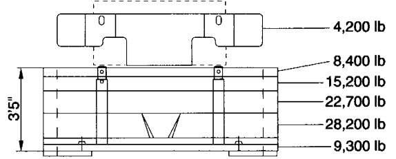
88,000 lb counterweight
