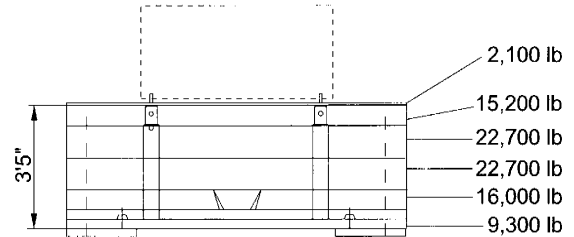
88,000 lb counterweight
